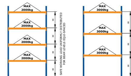
Europallets 800mm x 1200mm stored in 1100mm deep frames
