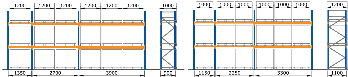
UK Pallets 1200mm wide x 1000mm can be stored 1200mm wide x 1000 deep in 900mm frames or 1000mm wide x 1200 deep in 1100mm frames
