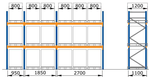
Europallets 800mm x 1200mm stored in 1100mm deep frames
